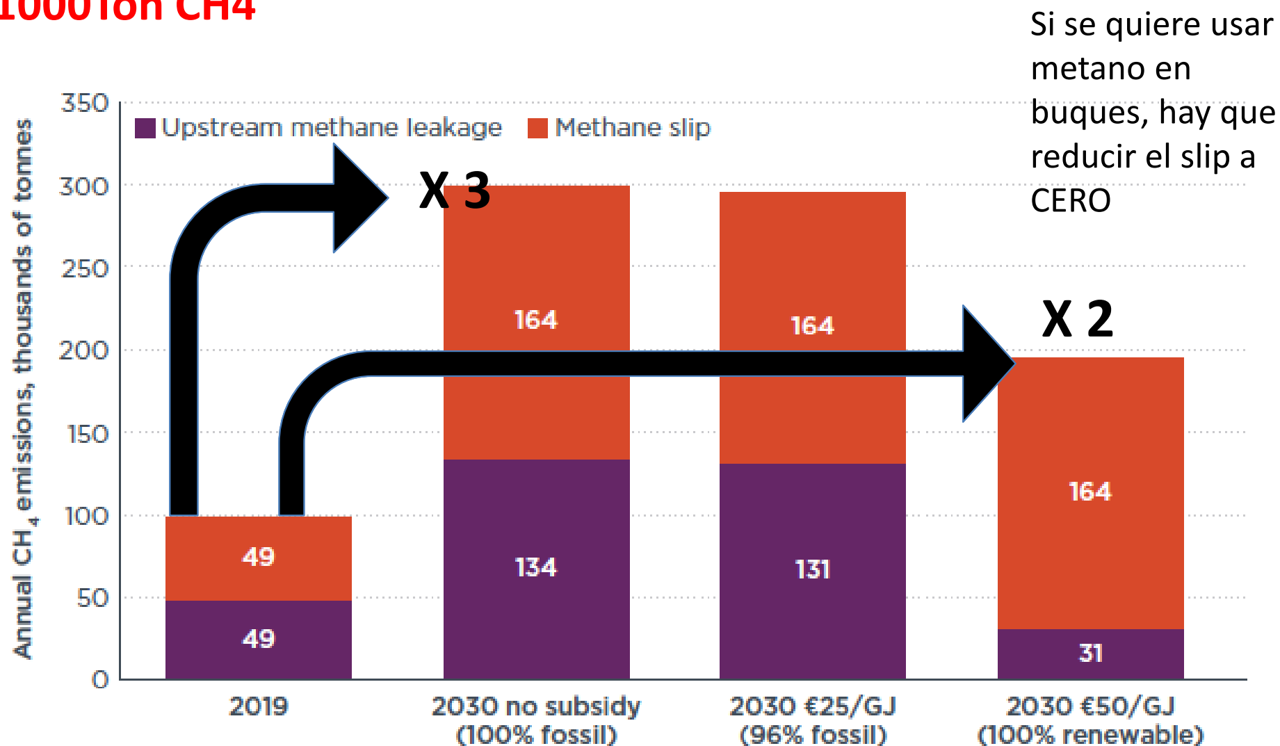
Figure 13. Estimated methane emissions from LNG-fueled ships trading with the European Union in 2019 and in three 2030 subsidy scenarios.
