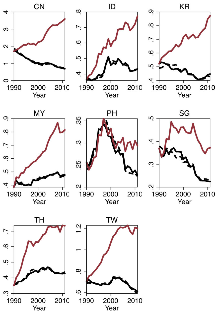
Figure 2. Observed and fitted carbon intensity.
